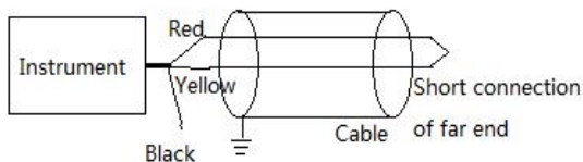
Figure 3.3.1 Connecting method of megameter
