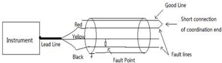
Figure 3.2.3 wiring of other-crossed fault
