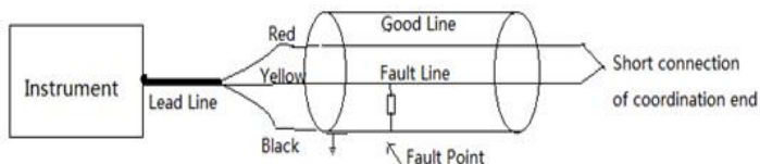
Figure 3.2.1 wiring of earthing fault
