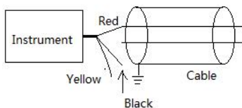
Figure 3.3.2 Connecting method of ohmmeter
