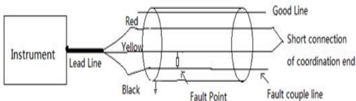
Figure 3.2.2 wiring of self-crossed fault
